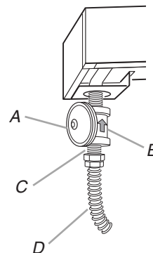
A. Gas pressure regulator B. Regulator - Must be installed with arrow pointing up to cooktop bottom. C. Adapter - Must have 1/2" male pipe thread. D. CSA Approved flexible stainless steel gas supply line
