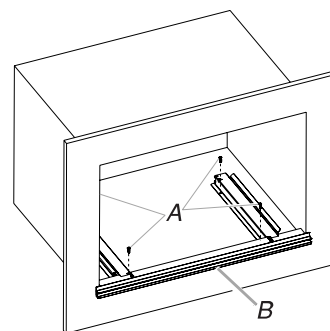
A. 3/4" flat-head screws B. Spacer kit assembly
