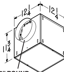
8" ROUND DUCT CONNECTOR
