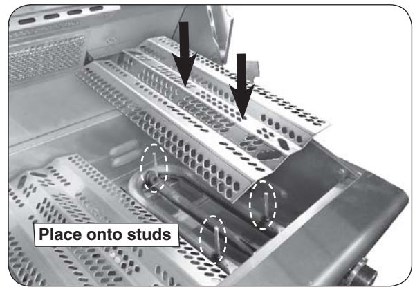
Fig. 16-1 Install vaporizer panels
