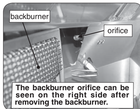
Fig. 29-4 Remove backburner
