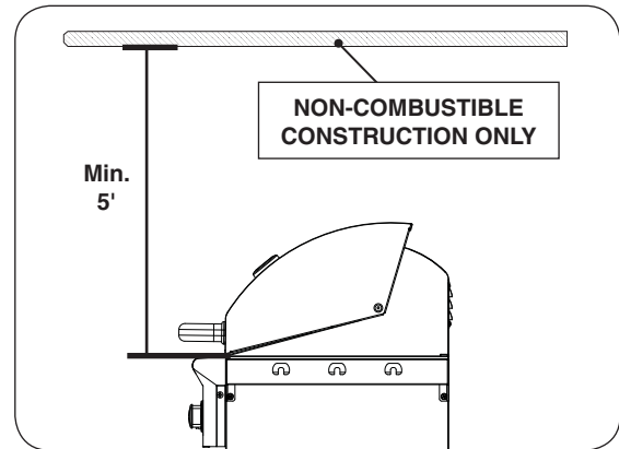
Fig. 10-1 Overhead requirements
