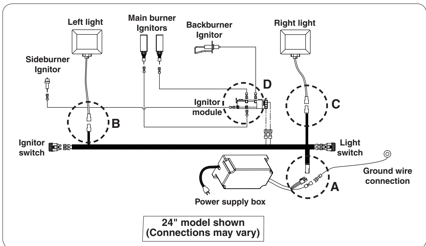
Fig. 32-1 - Wire diagram
