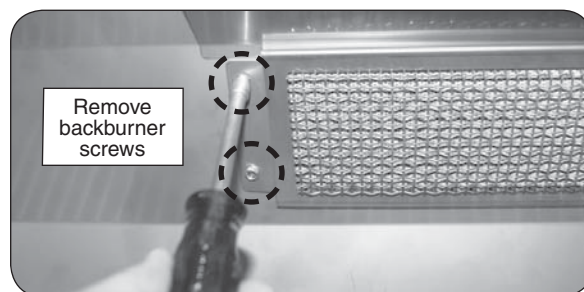
Fig. 29-3 Remove backburner mounting screws
