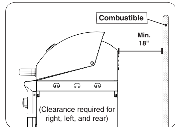
Fig. 10-2 Clearance 'A' Diagram
