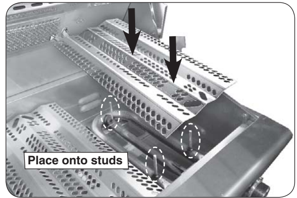
Fig. 16-1 Install vaporizer panels
