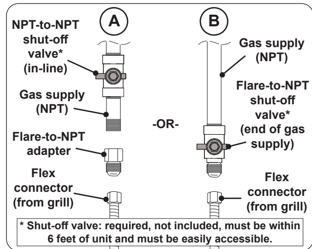
Fig. 23-1 Connecting to a gas line
