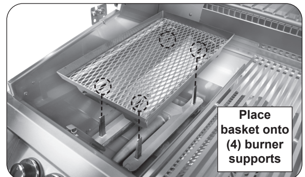
Fig. 36-3 Place basket onto burner
