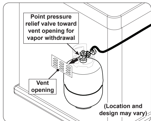
Fig. 7-2 Vapor withdrawal detail
