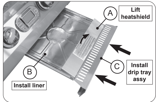
Fig. 25-1 Install drip tray
