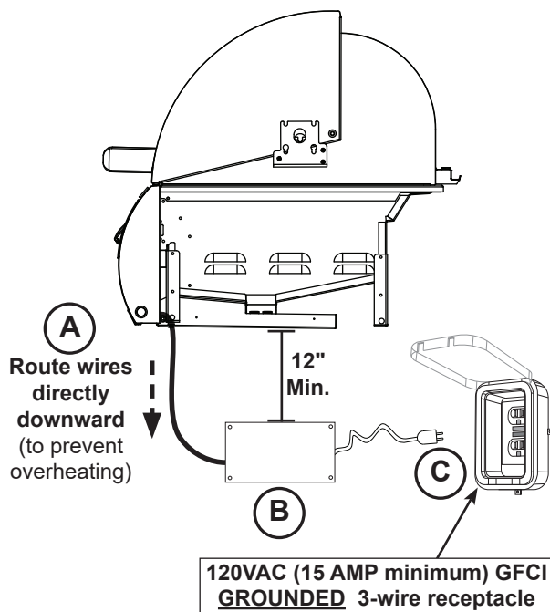
Fig. 26-1 Electrical installation
