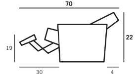
Side View (wall saver mechanism, fully reclined)
