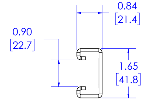
PROFILE VIEW 1:2
