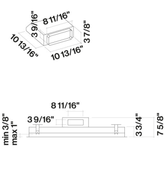
Side view with junction (optional)
