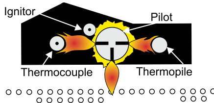
Front Burner Tube Top view of pilot flame
