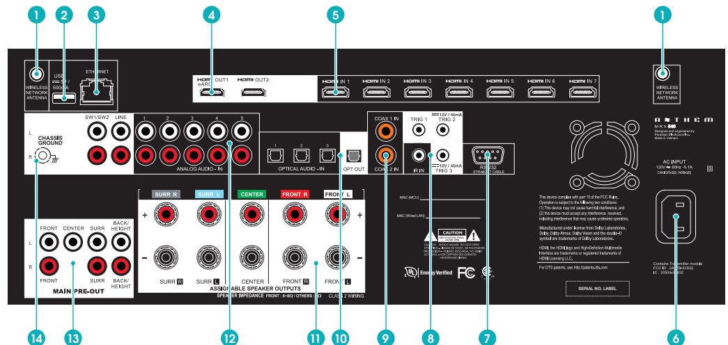
MRX 540 REAR VIEW
