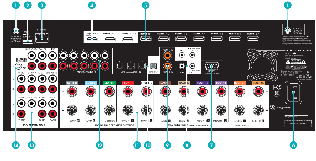
MRX 1140 REAR VIEW
