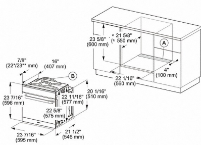
H 6000 E/B, 60 cm (Installation drawing) - USA
