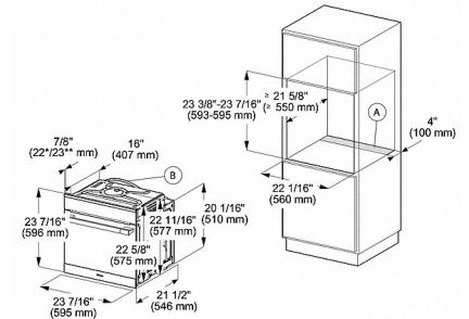
H 6000 E/B, 60 cm (Installation drawing) - USA
