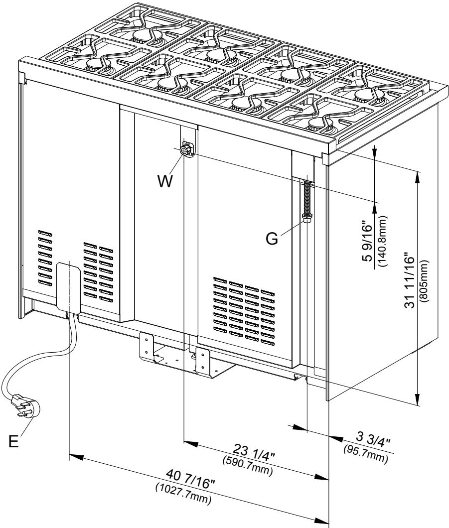
Rear view of HR 1954
