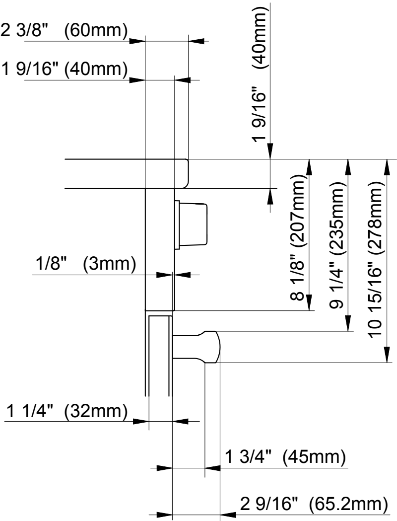
Detailed front side view of HR 1954
