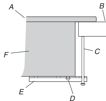
A. Cooktop B. Countertop C. 2½" (6.4 cm) clamping screw D. Attachment screw E. Bracket F. Burner box
