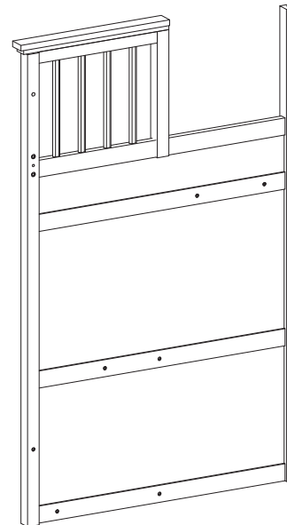
Inner Staircase Support Panel X 1
