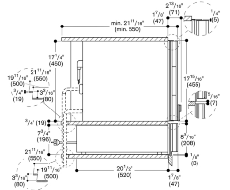
Side view WS 463 under BS, BM, CM
