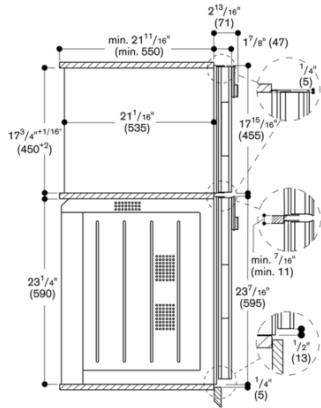
Side view of BM 450/451 above BO
