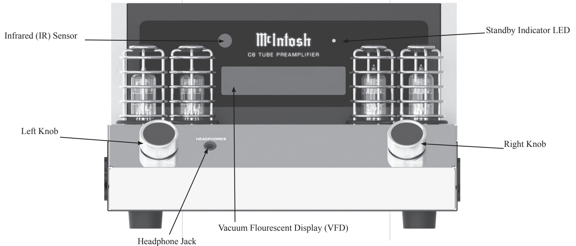
Figure 03– Front Panel
