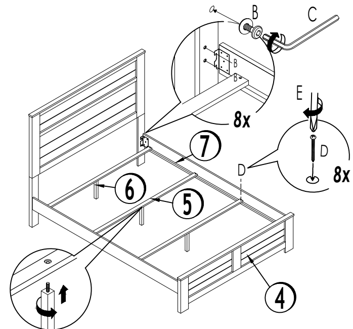
(BOX 2) - BOX OF SIDE RAIL
