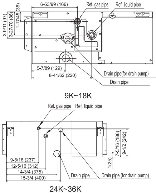
Fig. 4.1 The connection positions of the pipe
