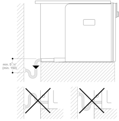
Drainage connection
