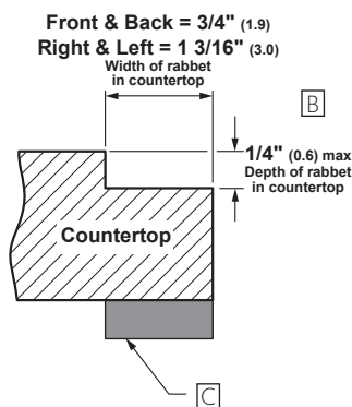
SECTION X-X Through countertop showing depth of rabbet for flush-mount
