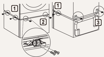
Attaching appliances to each other and snugging up the Main Washer
