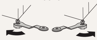
Attaching appliances to each other and snugging up the Main Washer
