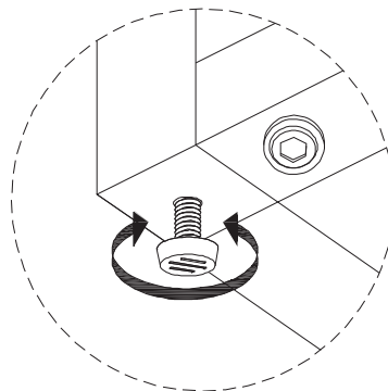
Adjustable Leveler
