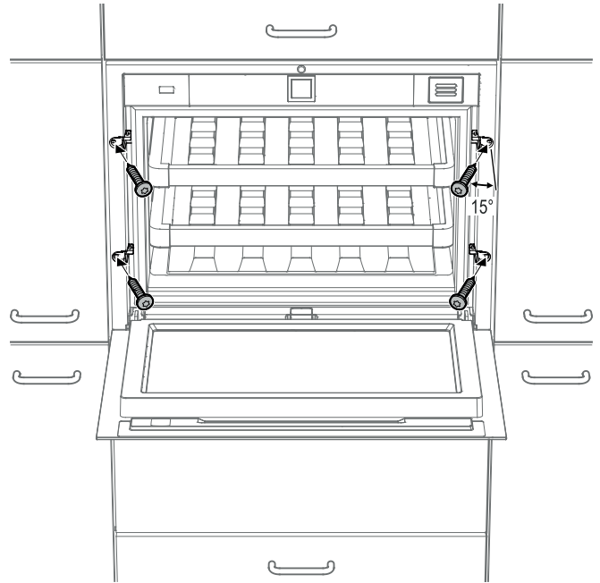
7. Secure the appliance to the kitchen unit using four screws (4 x 29).
