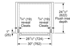
Flush installation Top view
